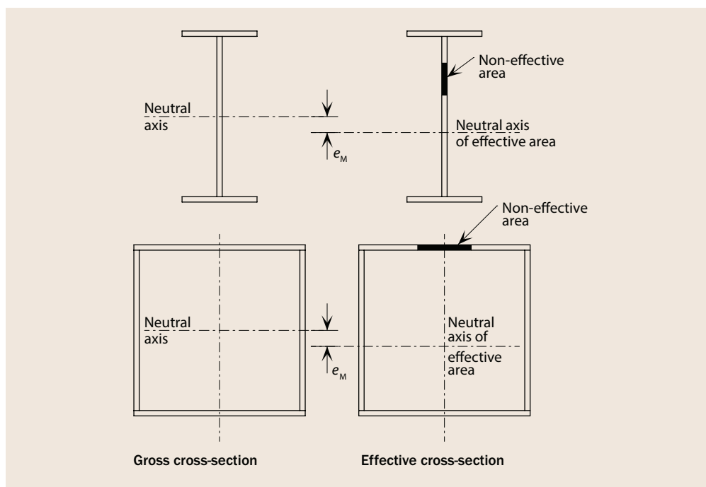
Figure 5.1 Class 4 cross-section subject to bending moment
