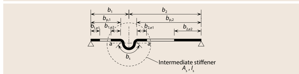
Figure 5.4 Intermediate stiffener
