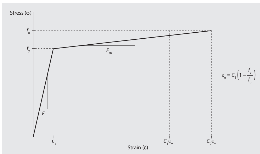
Figure D.1 CSM elastic, linear hardening material model
